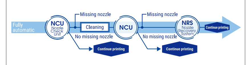
NCU (Nozzle Check Unit)
